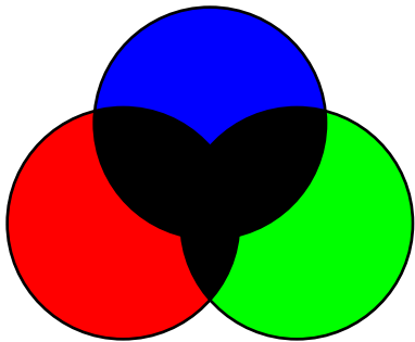
HPDF_BM_COLOR_BUM
