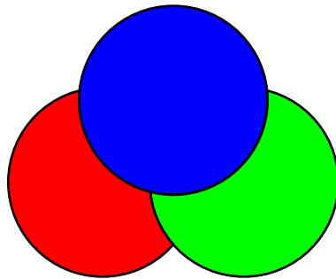
HPDF_BM_HARD_LIGHT
