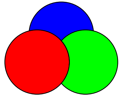
HPDF_BM_SOFT_LIGHT
