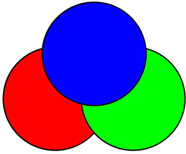
HPDF_BM_NORMAL
