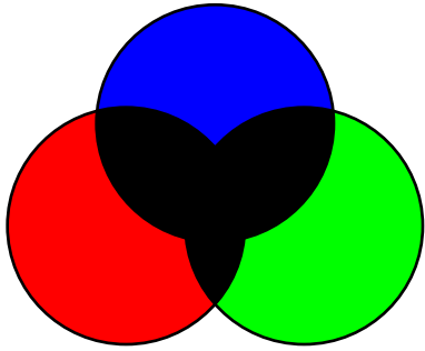
HPDF_BM_DARKEN
