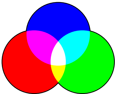
HPDF_BM_DIFFERENCE
