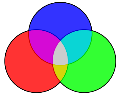
HPDF_BM_SCREEN alpha=0,8
