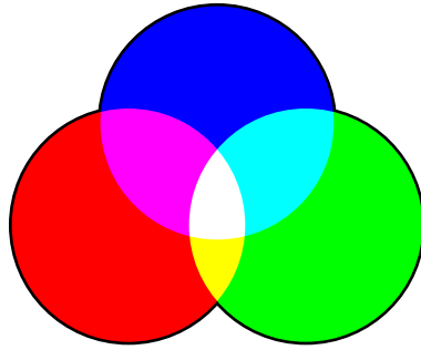
HPDF_BM_LIGHTEN
