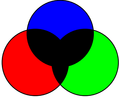
HPDF_BM_MULTIPLY
