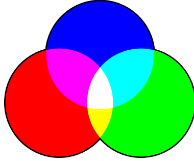
HPDF_BM_SCREEN
