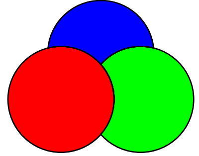
HPDF_BM_OVERLAY
