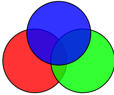
HPDF_BM_NORMAL alpha=0,8
