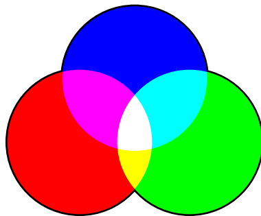
HPDF_BM_EXCLUSION
