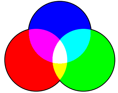
HPDF_BM_COLOR_DODGE
